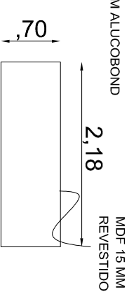
VISTA FRONTAL
